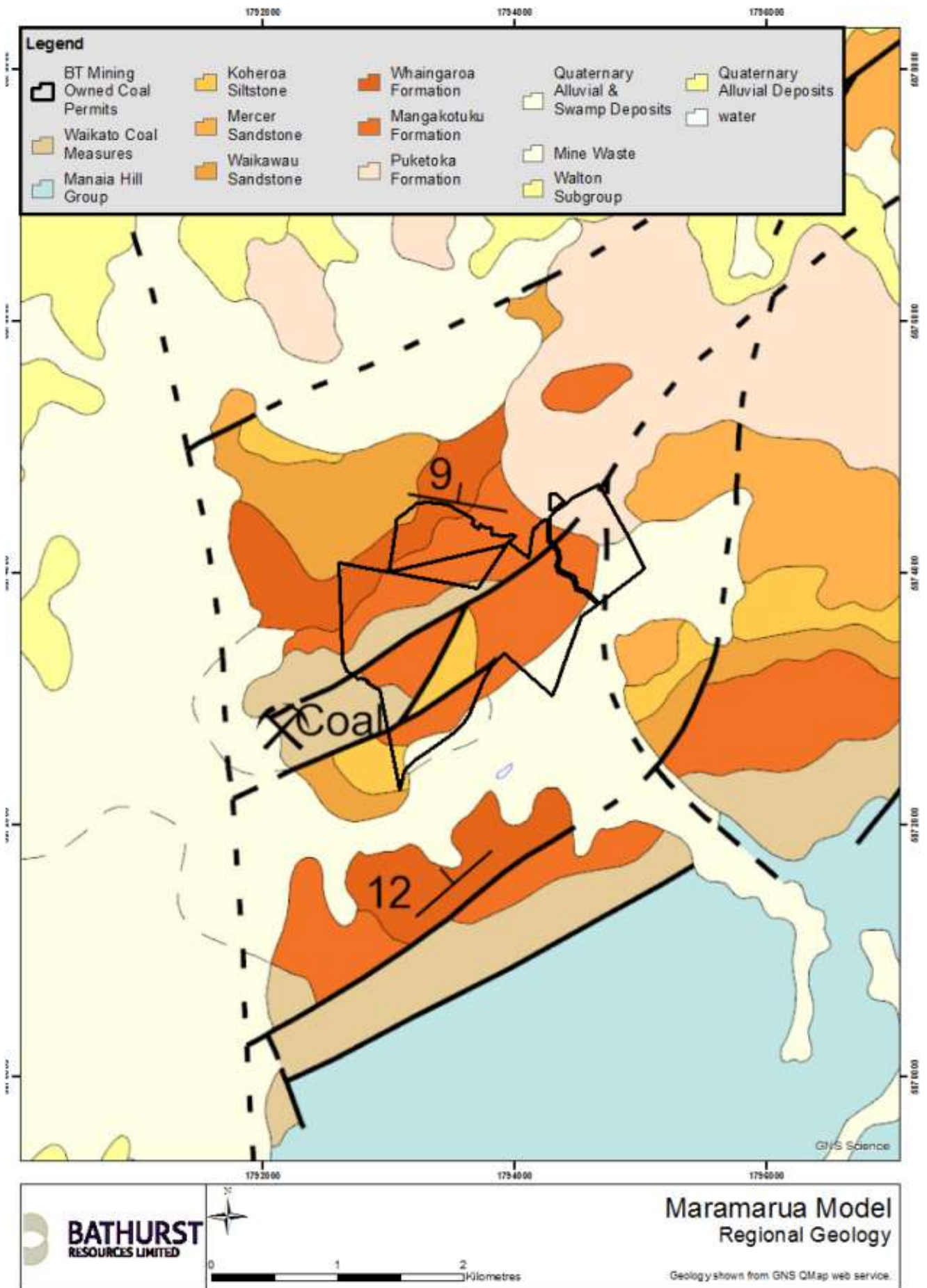
Figure 2 Regional Geology
