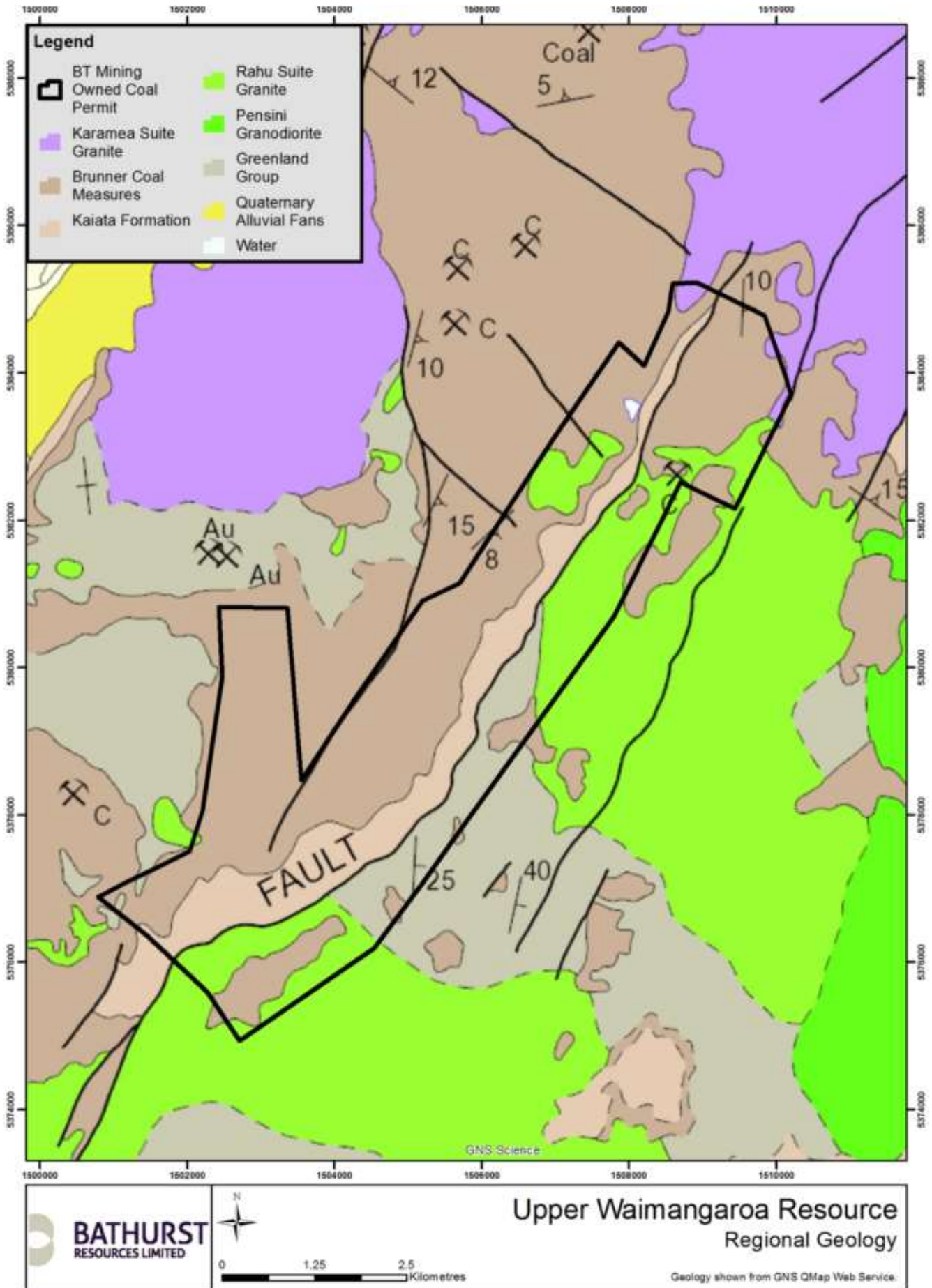
Figure 3 Regional Geology
